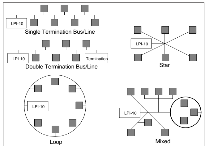
Typical Wiring Topologies Supported by the LPT-11 Link Power Transceiver
