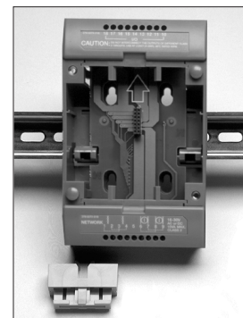
Type 1D Base Plate Front View
